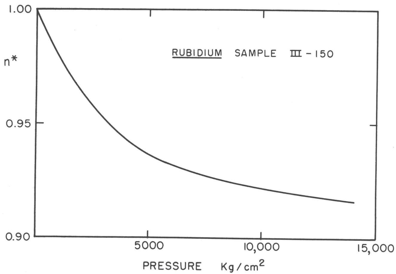
FIG. 3-13 n^* , NORMALIZED ELECTRONS/ATOM VS. PRESSURE
